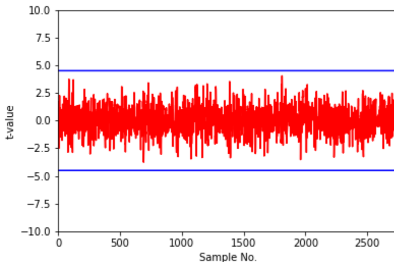
Figure 1 -Photon-Beetle_first_order TVLA (10 million traces)
