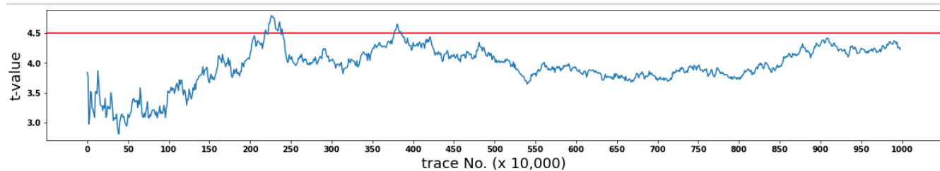
Figure 2 - Photon-Beetle_first_order maximum t-value vs. number of traces (x 10,000)
